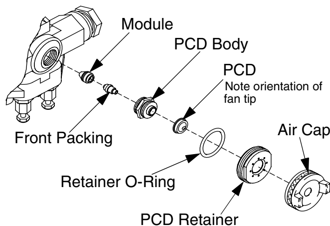
FIG. 30: Install Mixing Module
