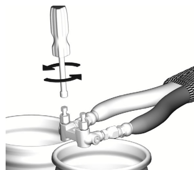
FIG. 21: Open Manual Valves
