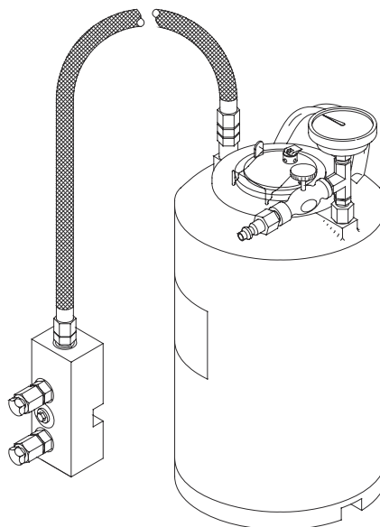
FIG. 23: 3-Gallon Gun Service Kit For more information about the 3-Gallon Gun Service Kit, see Manual 311341.
