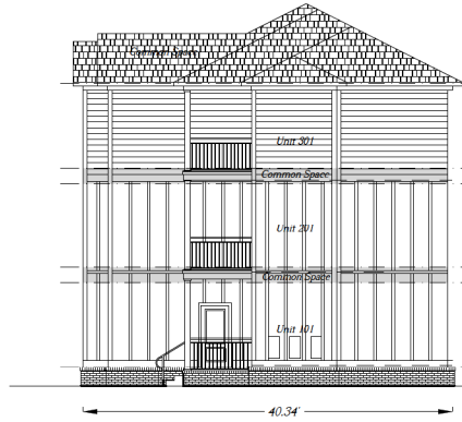
East Elevation
