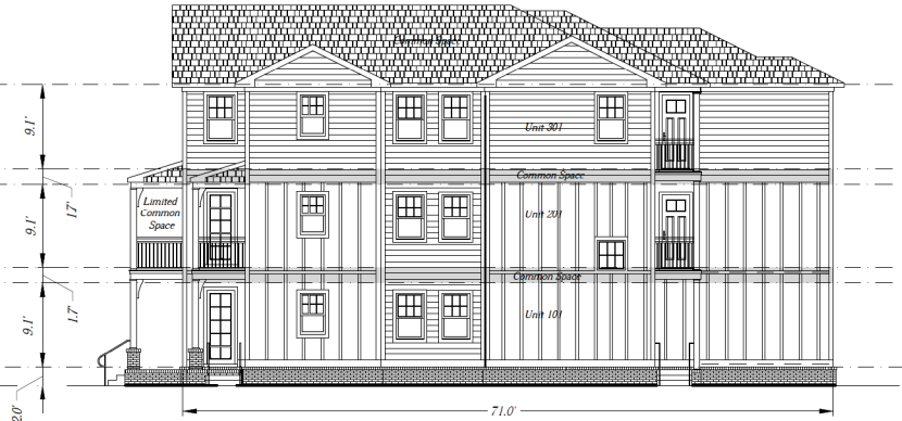
North Elevation
