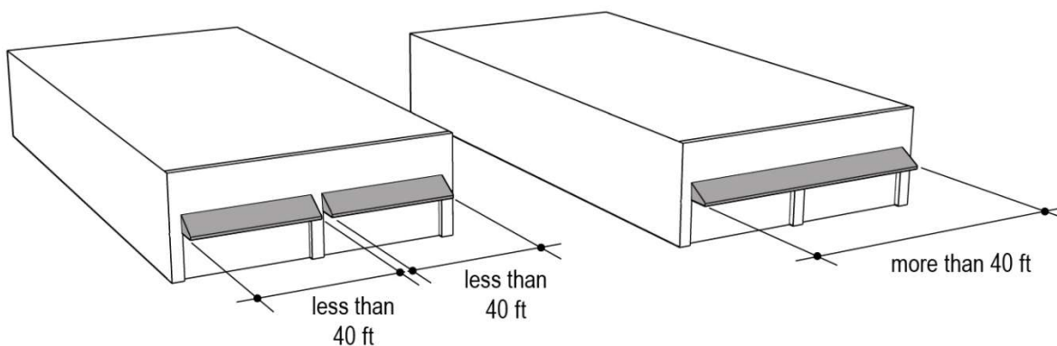
Figure 6-4 Awning length
