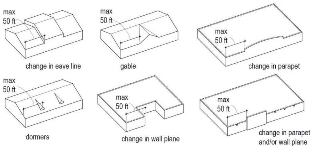
Figure 6-3 Roof articulation
