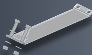
Band Clamp
